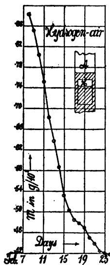
FIG. 5.—Loss of mass of gas in diver in lapse of days. Diffusion of hydrogen into air.
